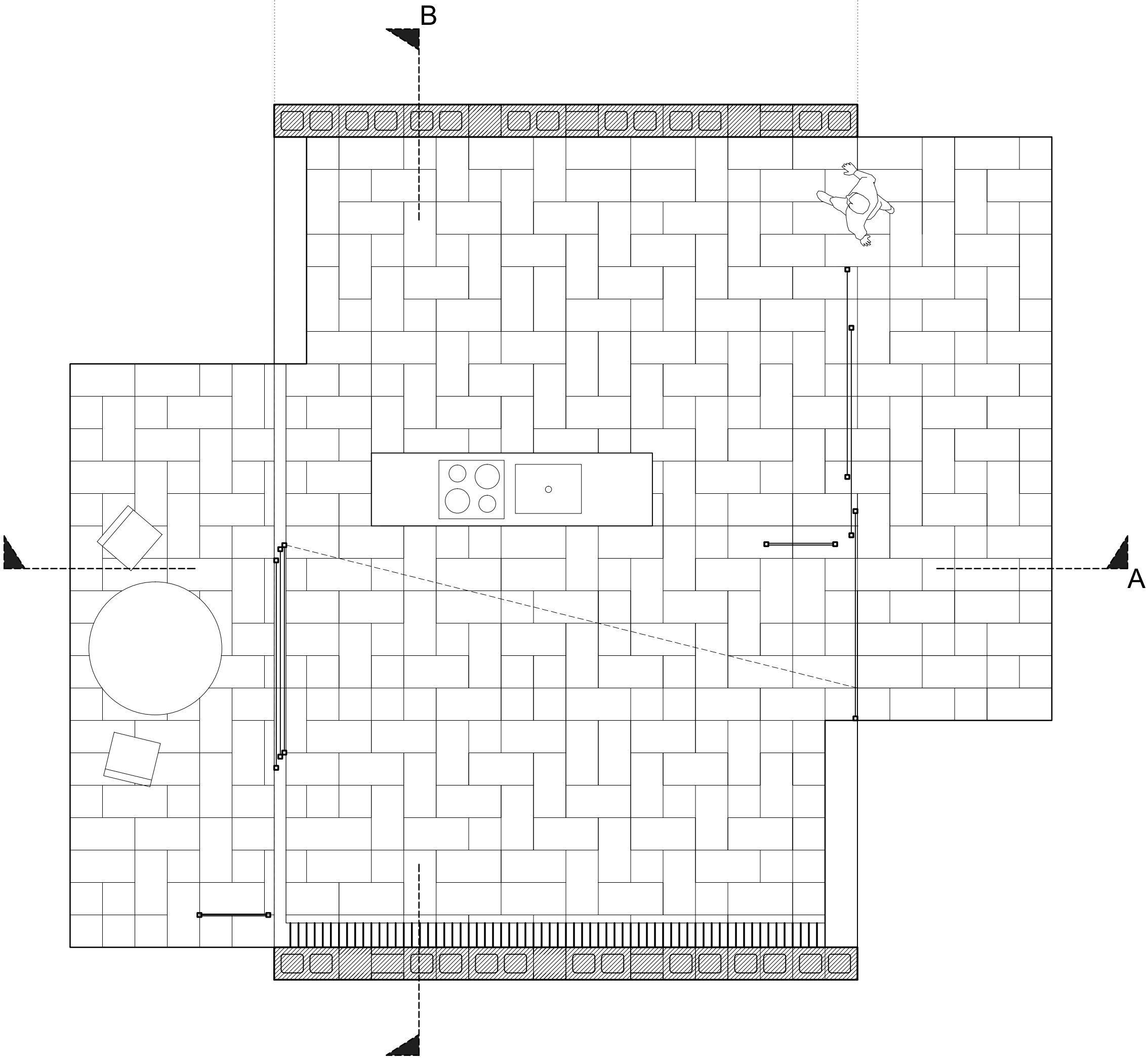
GROUND PLAN 1/2"=1'-0"
